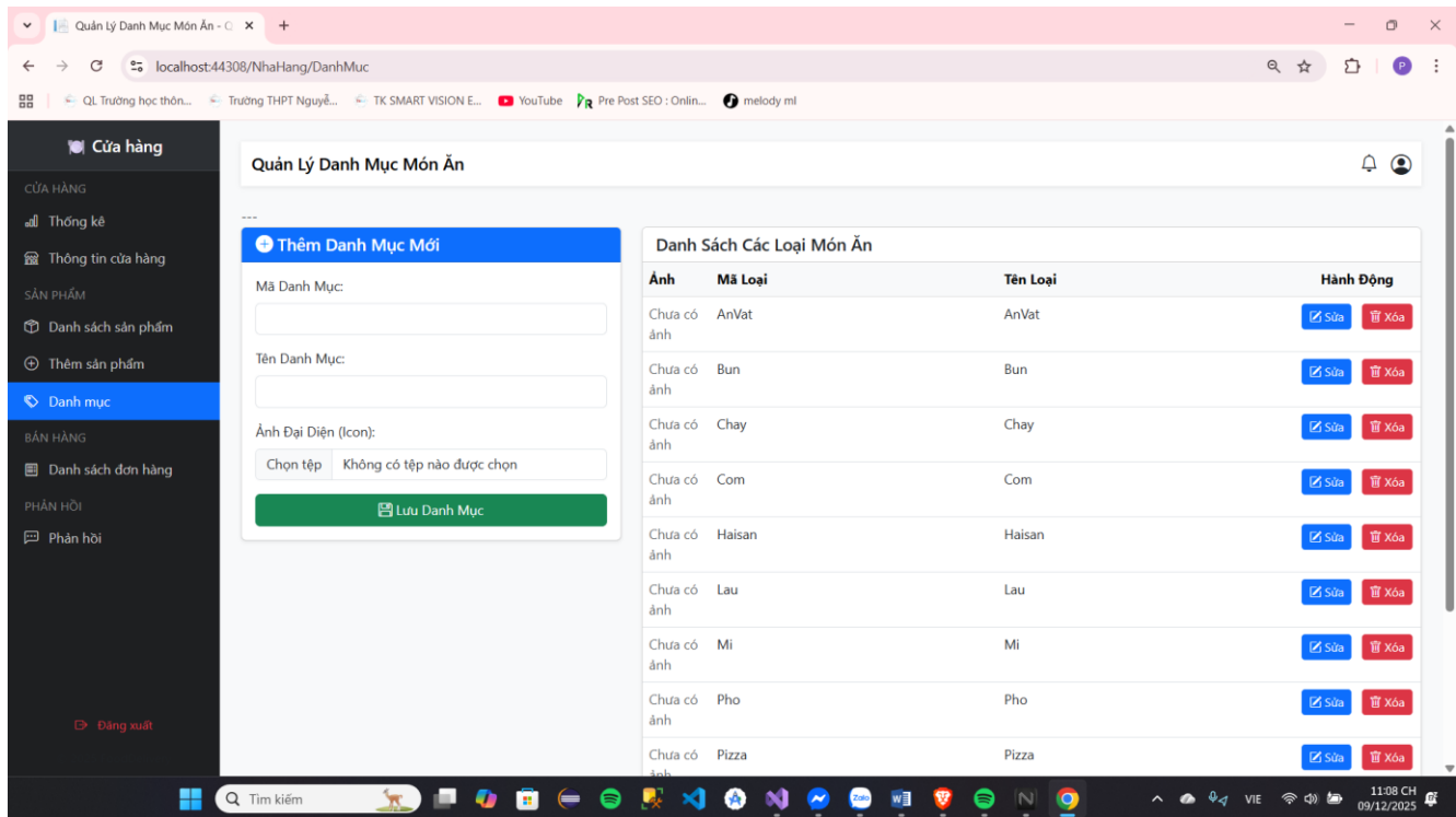
Image 32: Restaurant Directory
